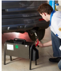
Wireless transmission smoke meter.
