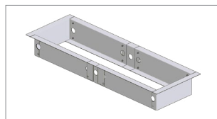
Installation frame.
